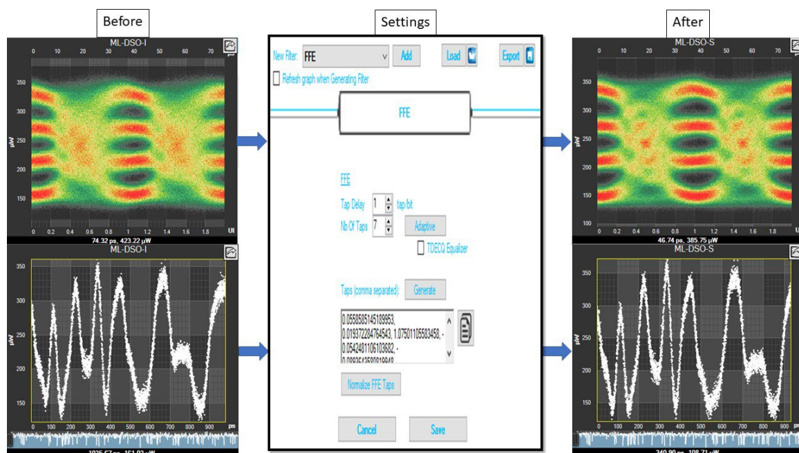
Figure 33: FFE Filter
