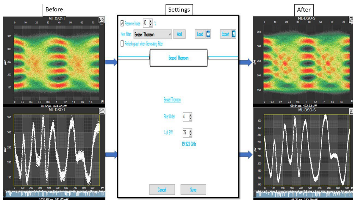
Figure 37: Filter + Preserve Noise
