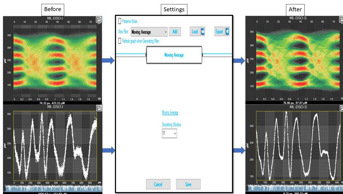
Figure 34: Moving Average Filter
