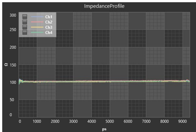
Figure 8 Impedance profile Graph
