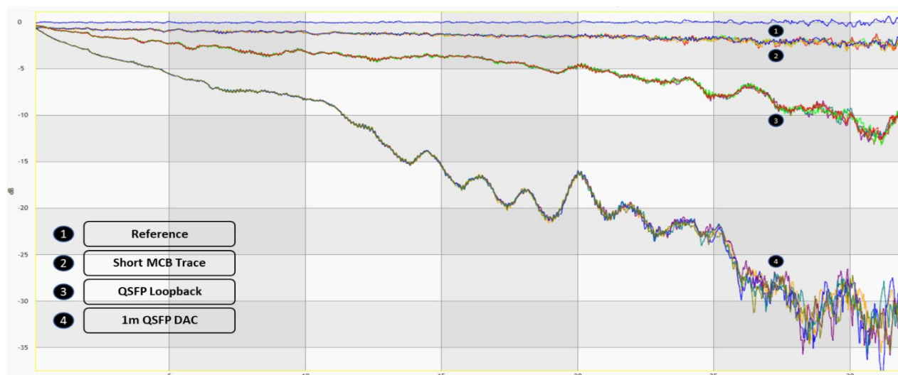
Figure 15 S21 Measurement
