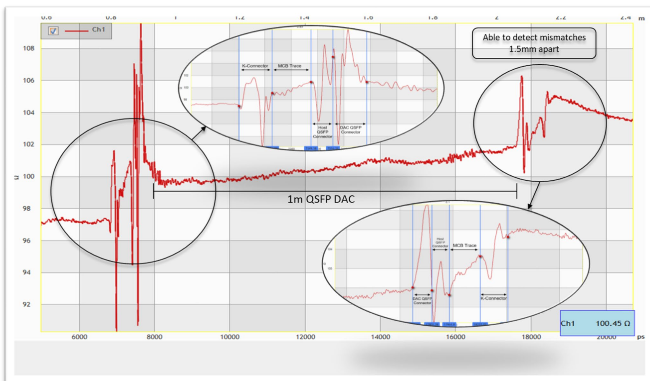
Figure 10 TDR measurement
