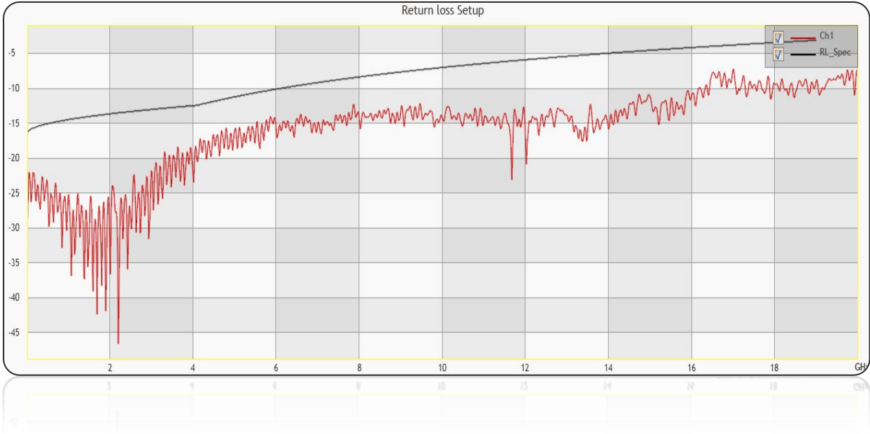
Figure 24: Return Loss Mask
