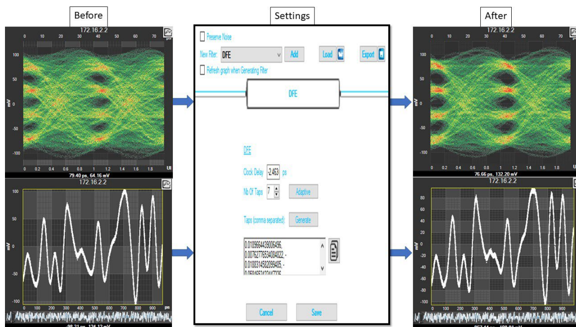
Figure 32: DFE Filter
