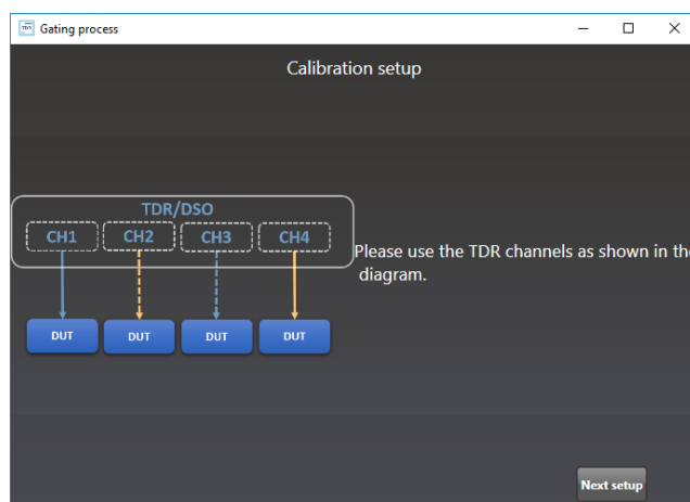
Figure 5 Calibration Wizard
