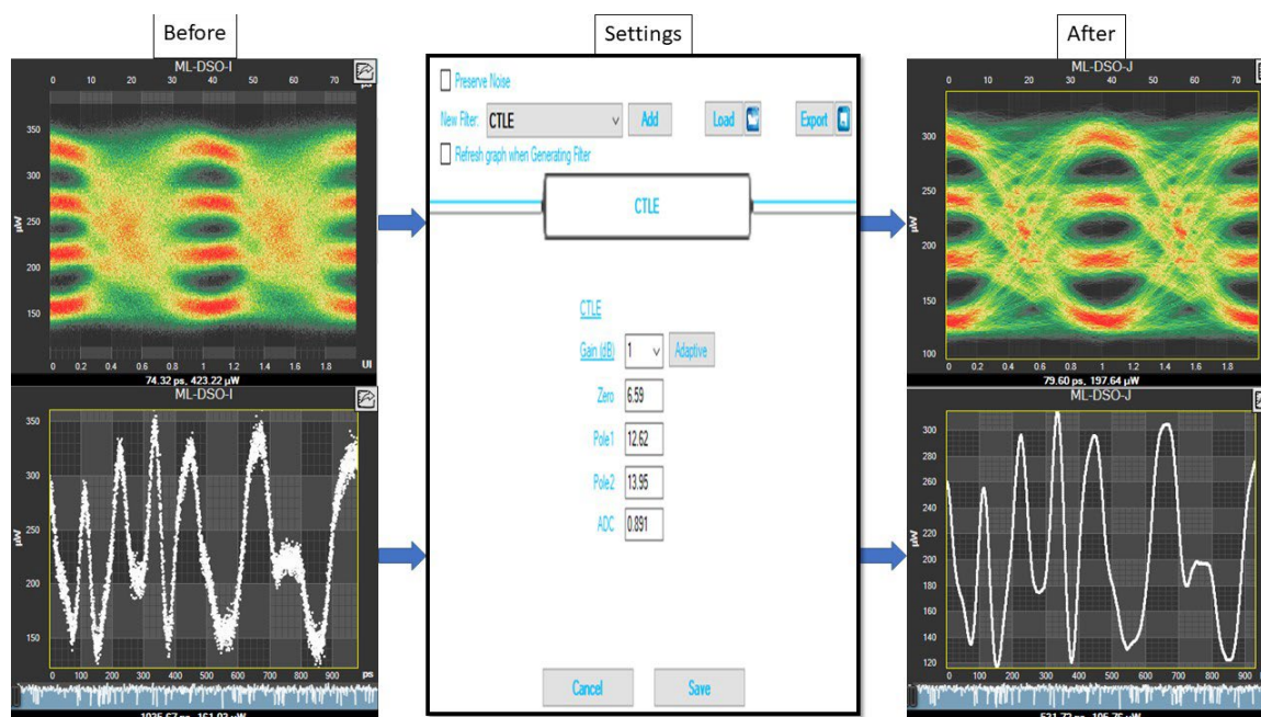
Figure 30: CTLE Filter
