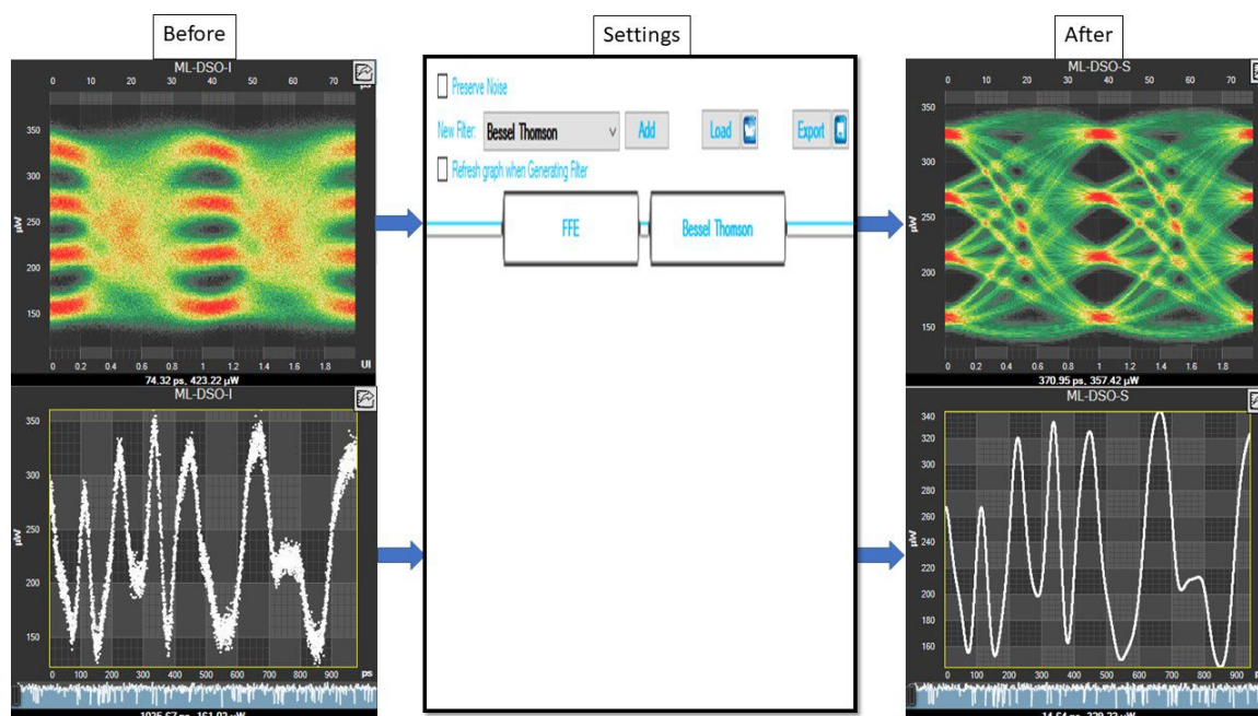
Figure 36: Multiple Filters
